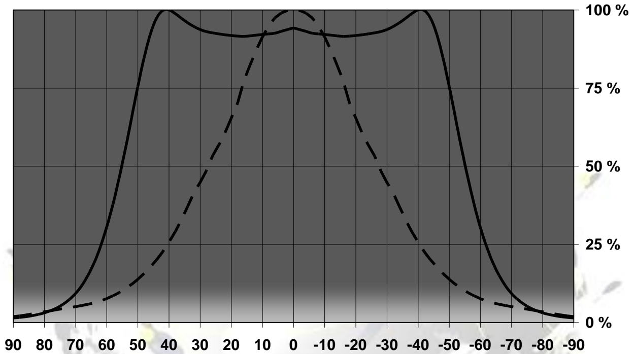
Relative Intensity of C11244_Strada-DN-N83
