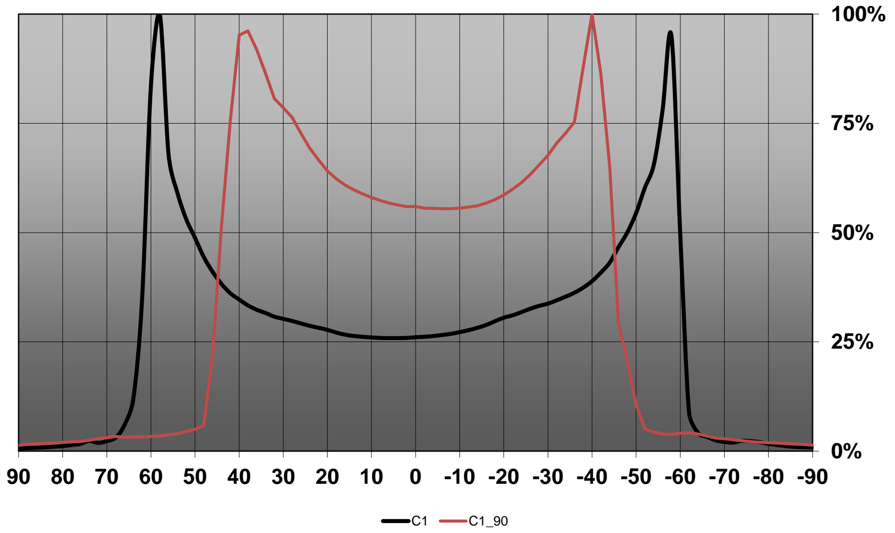
Relative intensity of CA16755_IRIE-A_(Luxeon_IR_2720)
