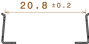
Clip reference distance after soldering
