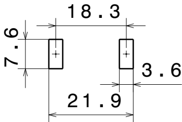
Recommended PAD design
