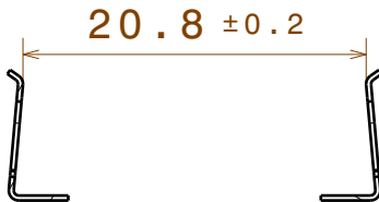
Clip reference distance after soldering
