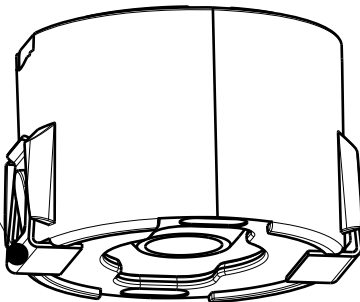
C18696_SOLDER-CLIP-2 Bottom of solder clip underneath holder Opening of solder clip facing holder
