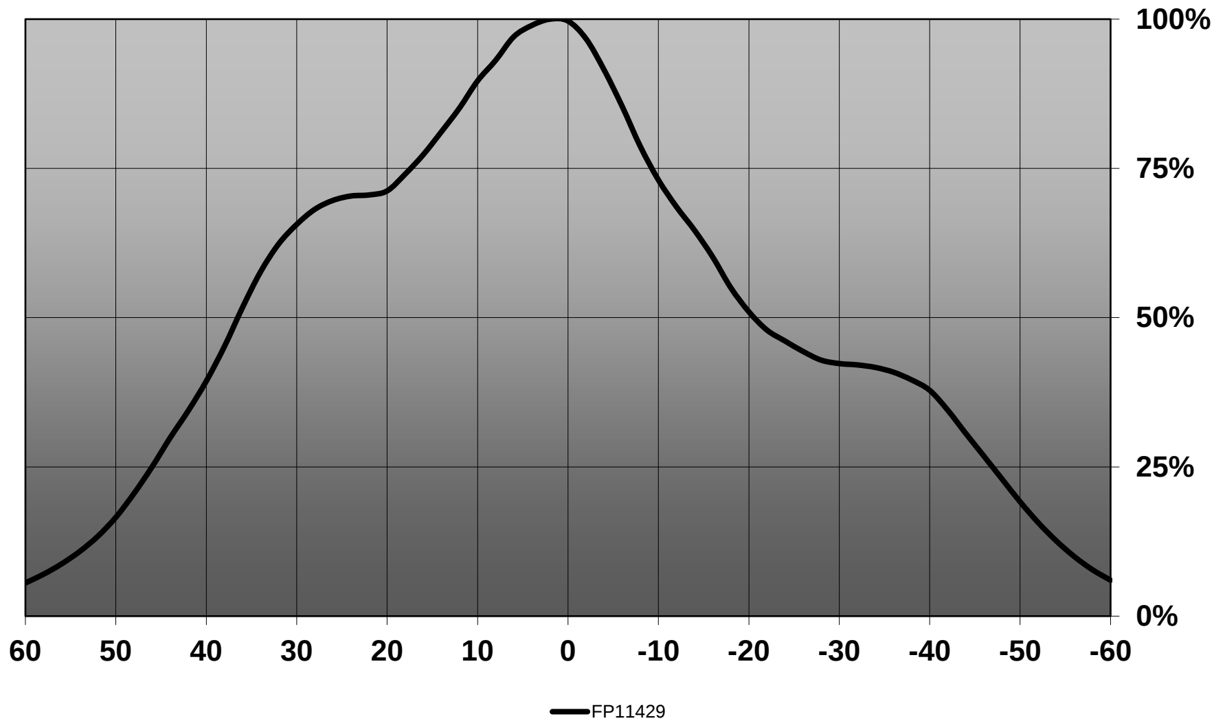
Relative intensity of FP11429_LISA2-WWW-PIN_(SFH_4180S)
