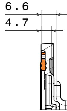
Section view A-A
