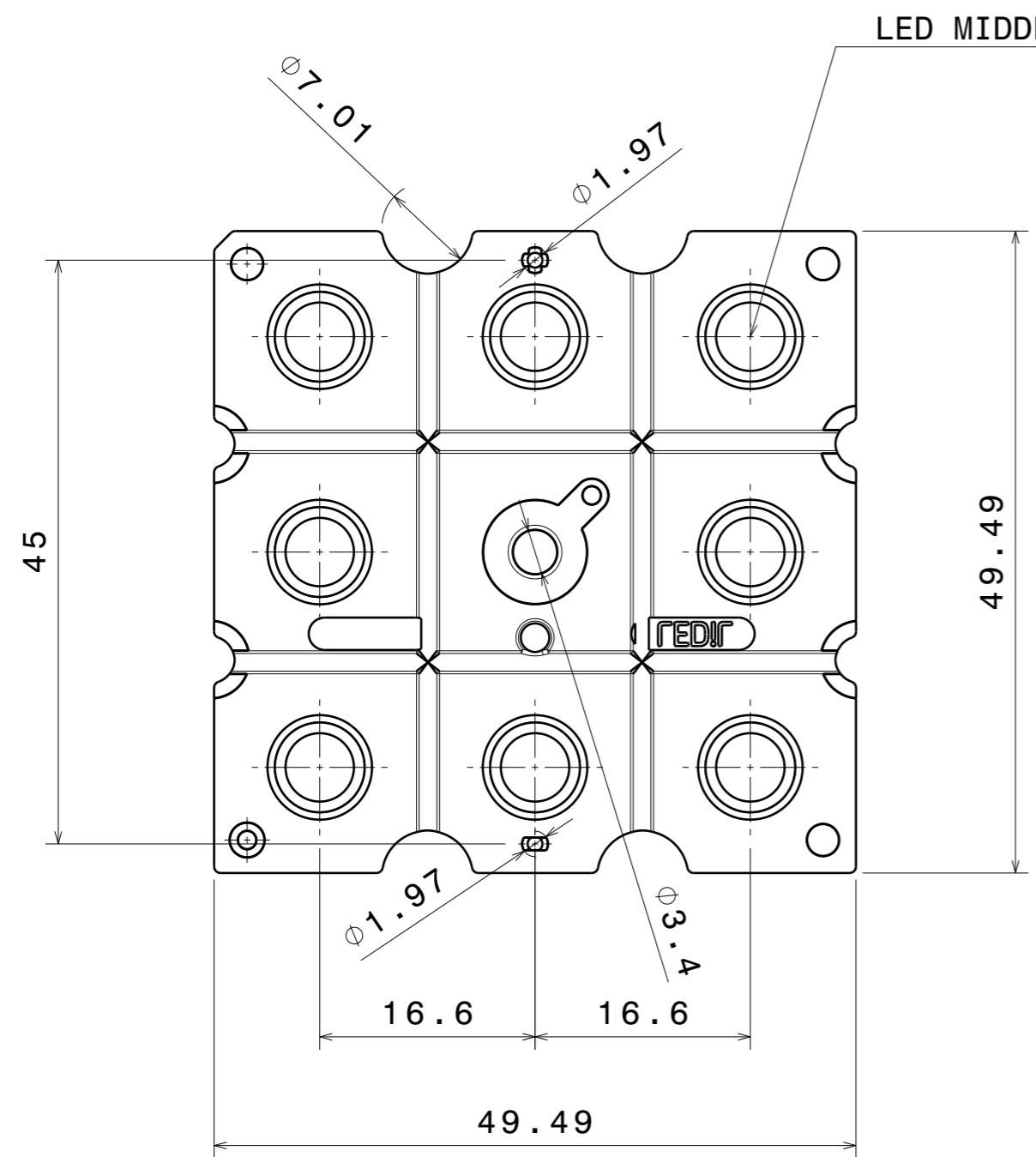
Front view
