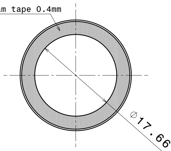
Bottom view with Tape
